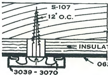
EXTRUDED MOULDINGS FOR STRUCTURAL GLASS (ALUMINUM AND BRONZE)
